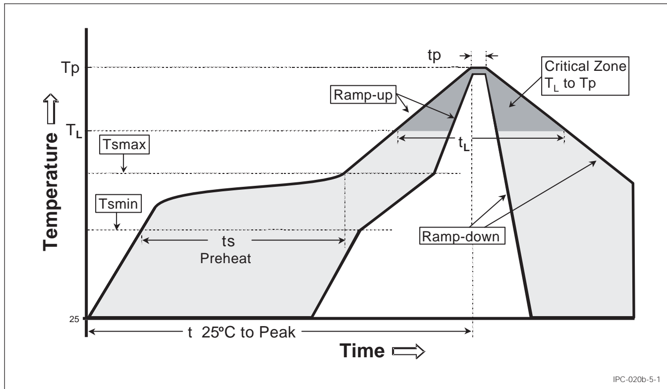
Figure 5-1 Classification Reflow Profile
